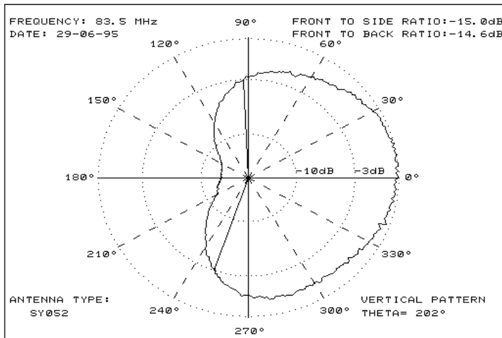
VERTICAL PATTERN
