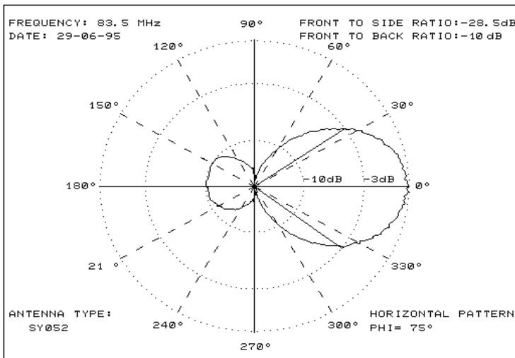
HORIZONTAL PATTERN
